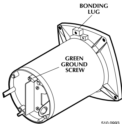
Figure 3 – Typical ground screw and bonding lug locations.
